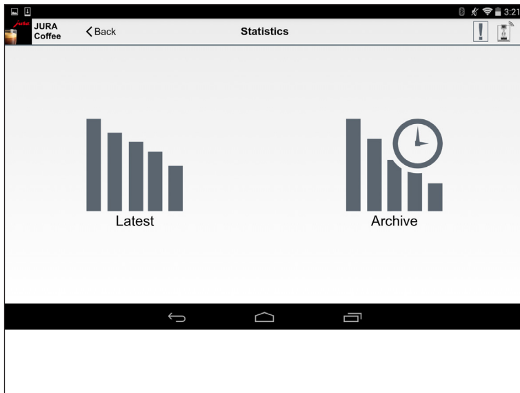
Fig. 15: Statistics
