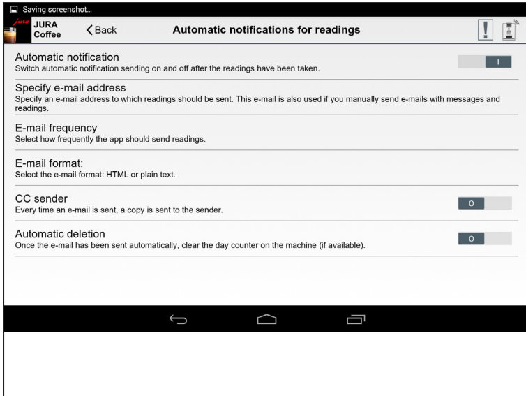
Fig. 37: Automatic notification
