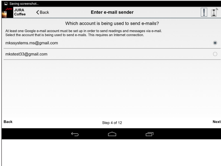
Fig. 43: E-mail configuration
