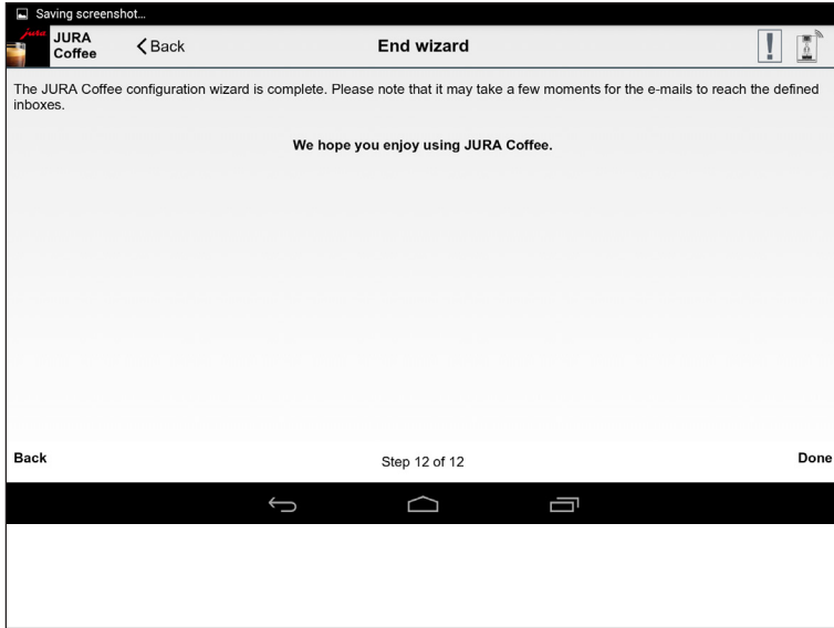
Fig. 49: Ending wizard
