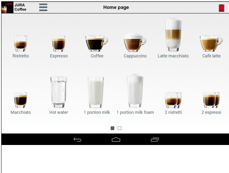
Fig. 1: Home page
