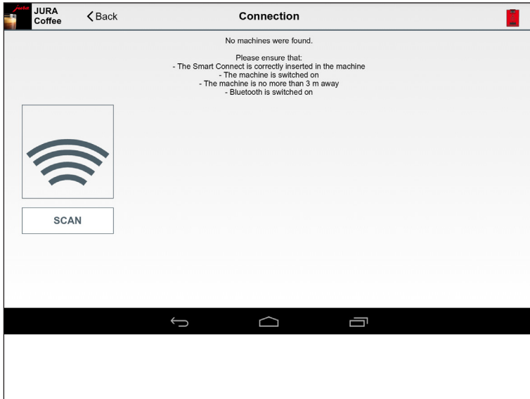
Fig. 2: Connection screen
