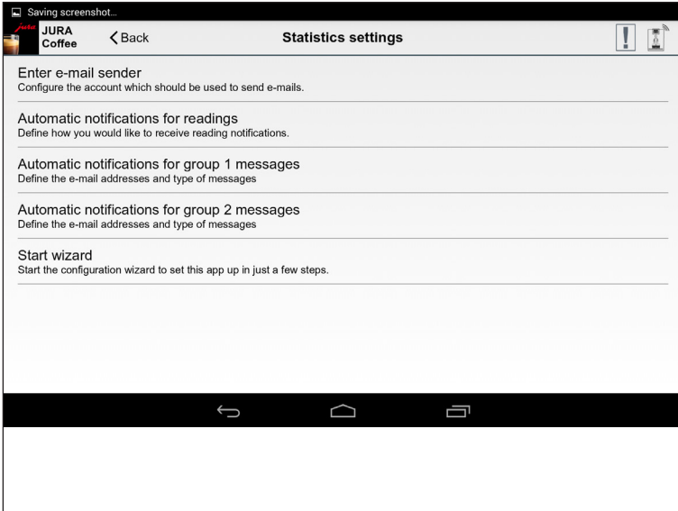
Fig. 34: Statistics settings
