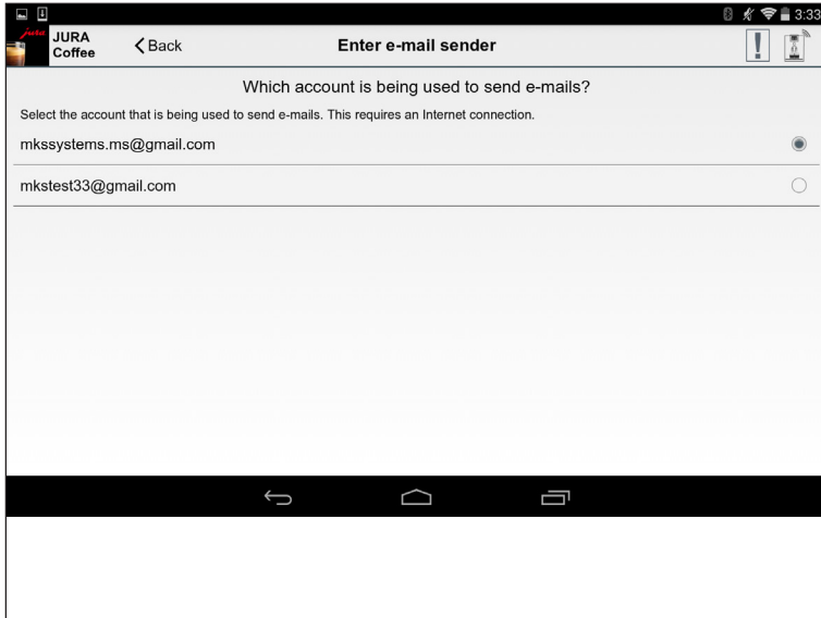
Fig. 35: E-mail settings
